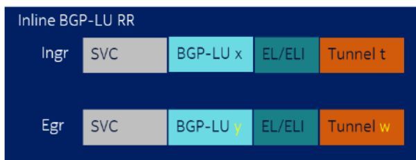
Figure 2: Inline BGP-LU RR
