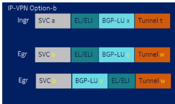
Figure 3: IP-VPN Option B
