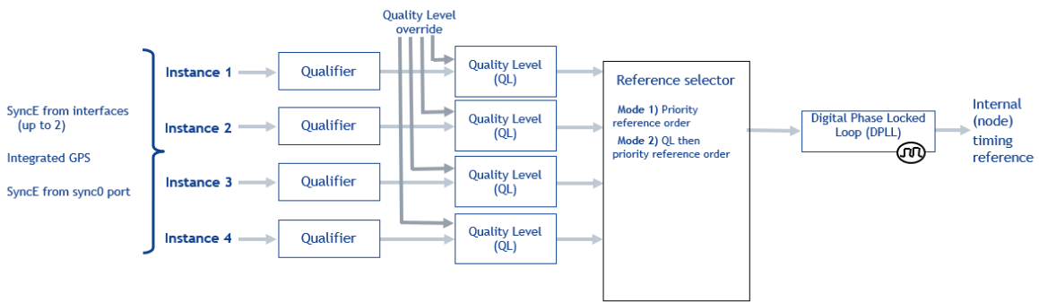
Figure 3: Logical mode of the synchronization reference selection (7730 SXR-series)
