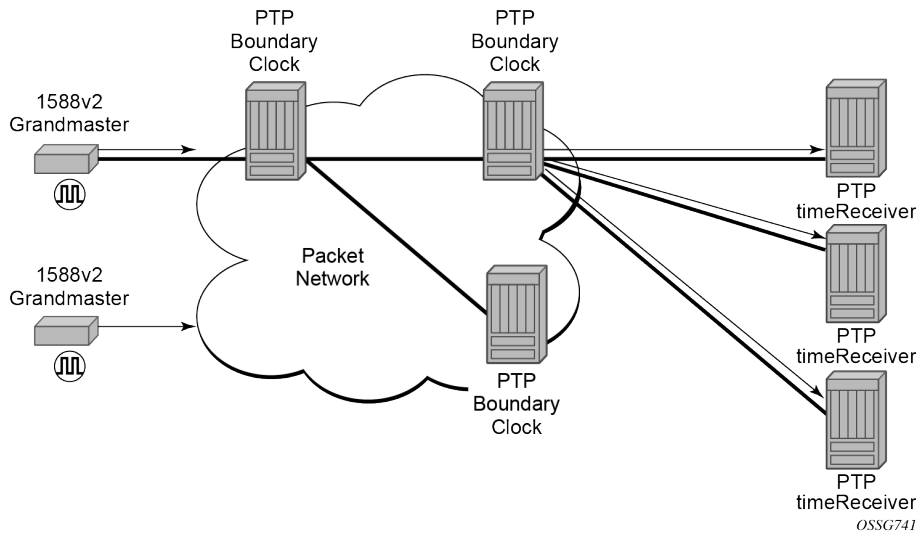
Figure 10: PTP boundary clock
