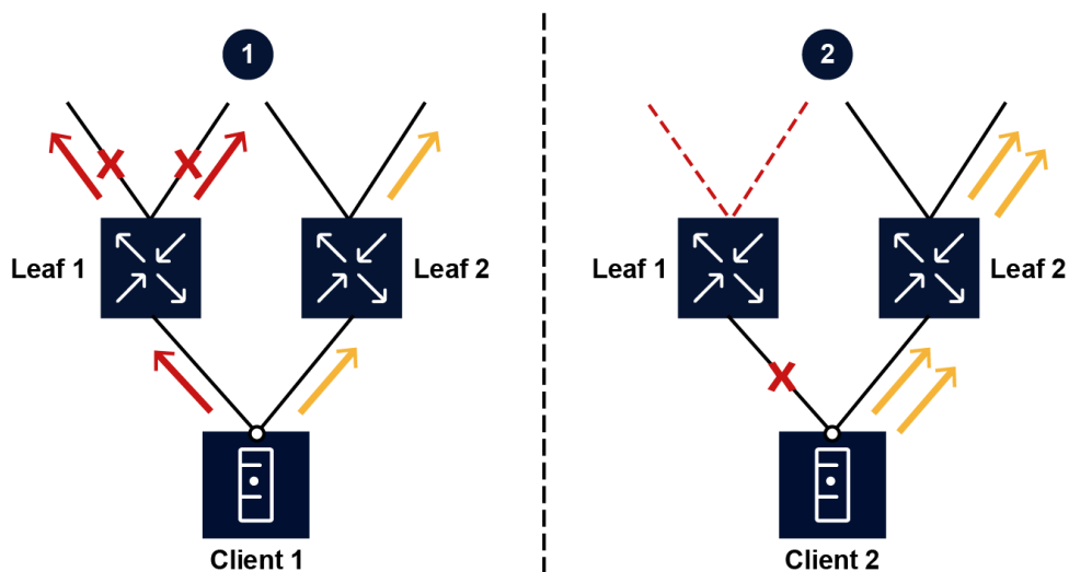
Figure 4: Using an oper-group to prevent traffic black-holing
