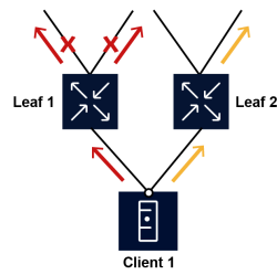
Figure 3: Traffic disruption when a leaf loses connectivity to upstream spines
