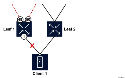
Figure 5: Disabling downlink based on uplink state
