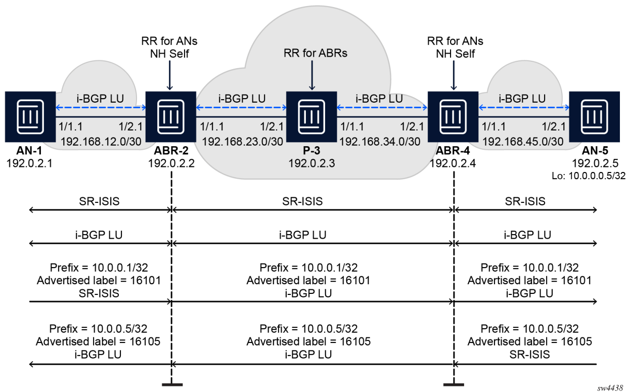
Figure 4: Segment routing with BGP-LU prefix SID topology - SR-ISIS/iBGP-LU domains
