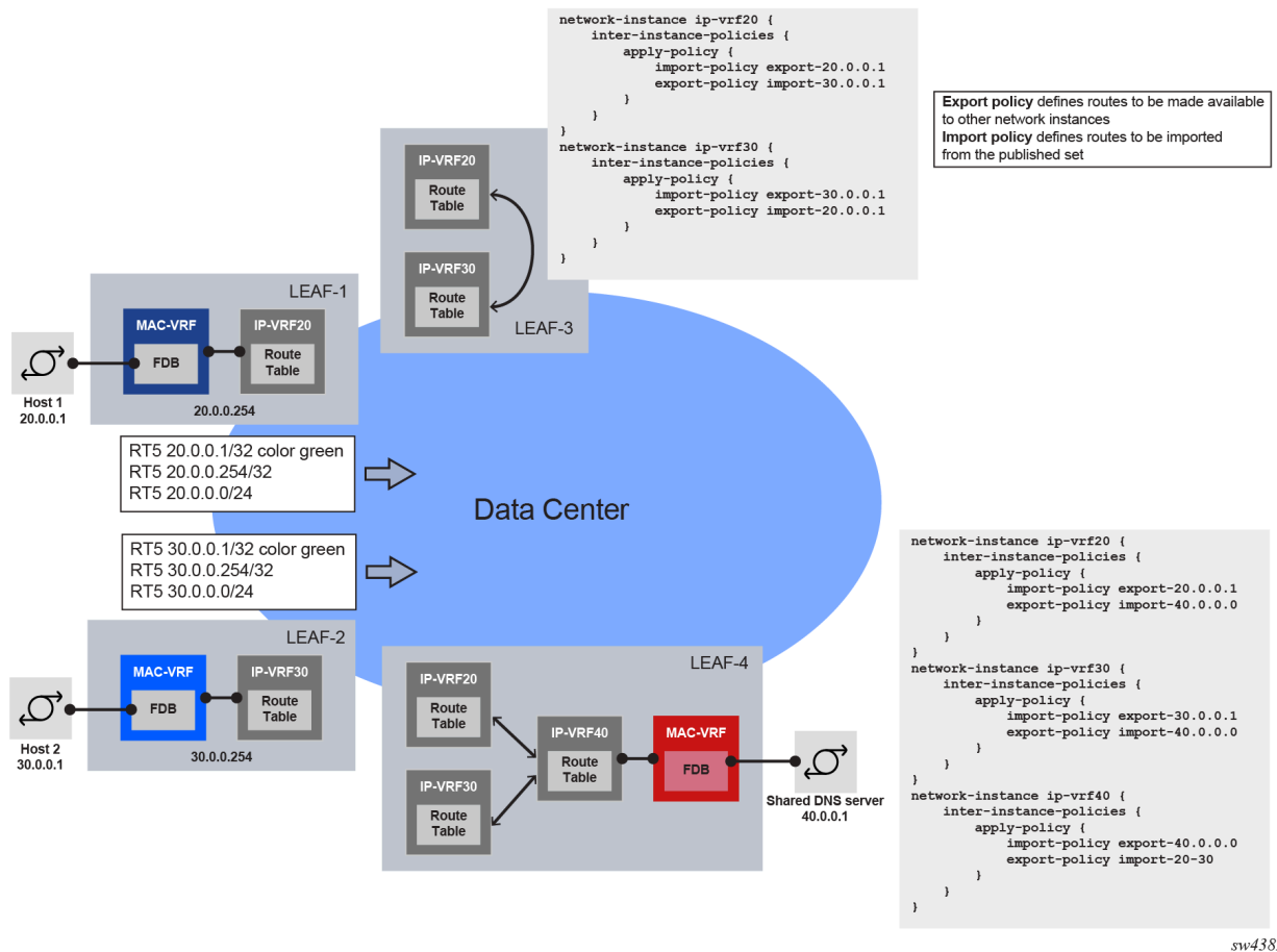
Figure 1: Network-instance route leaking
