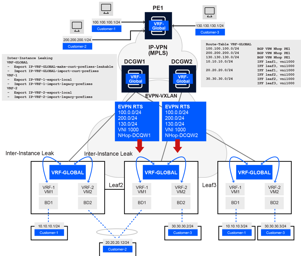
Figure 2: Network-instance route leaking example
