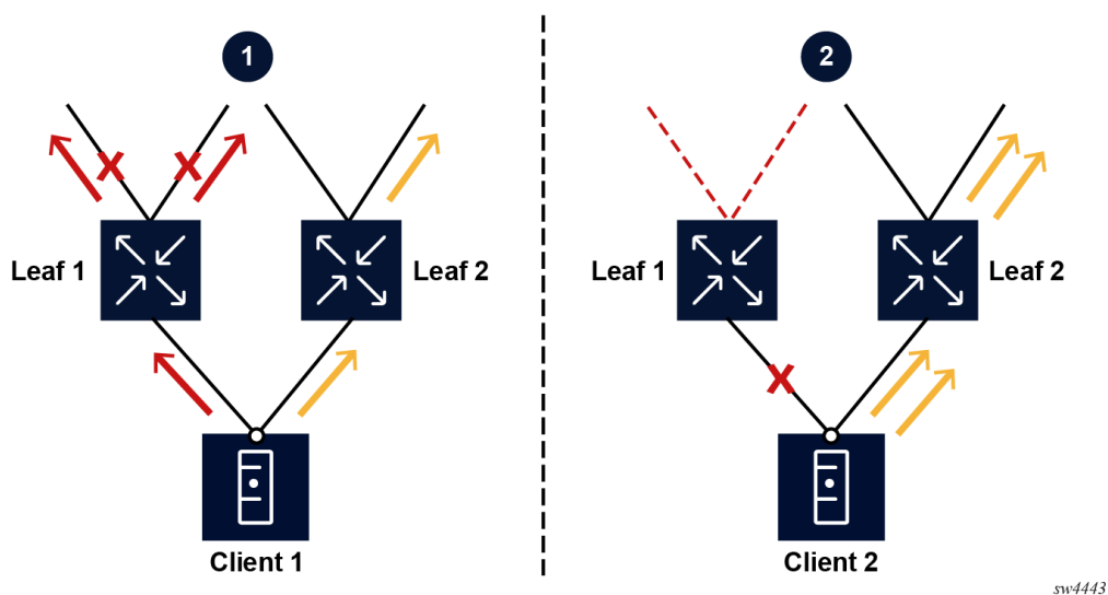
Figure 4: Using an oper-group to prevent traffic black-holing
