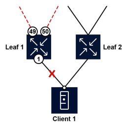
Figure 5: Disabling downlink based on uplink state
