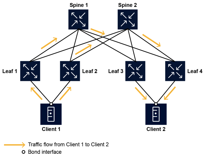
Figure 2: Clos topology with multi-homed clients
