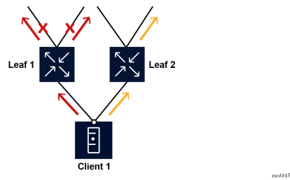
Figure 3: Traffic disruption when a leaf loses connectivity to upstream spines
