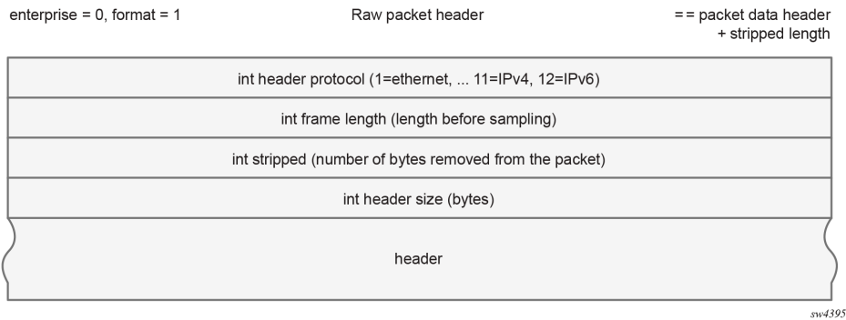
Figure 8: Raw packet header
