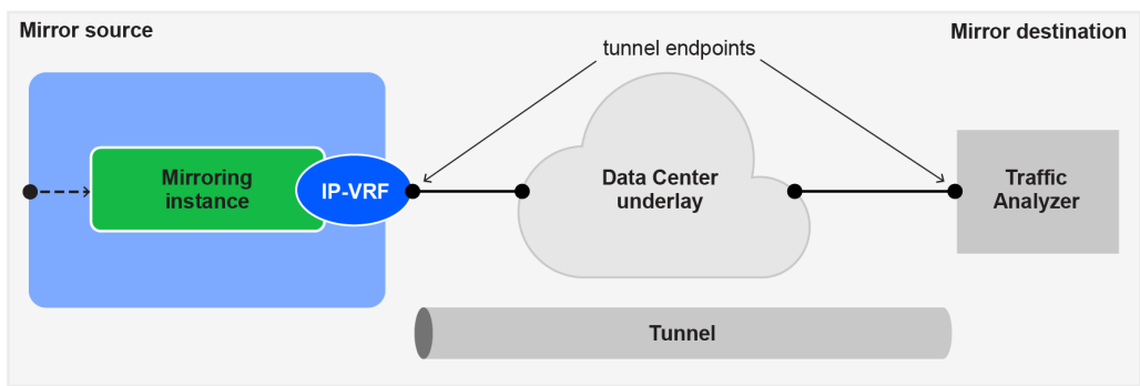
Figure 2: Remote mirroring
