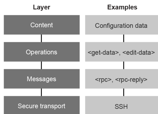
Figure 2: NETCONF layers
