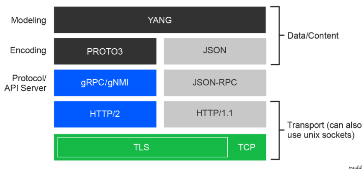
Figure 1: RPC-based interfaces in SR Linux
