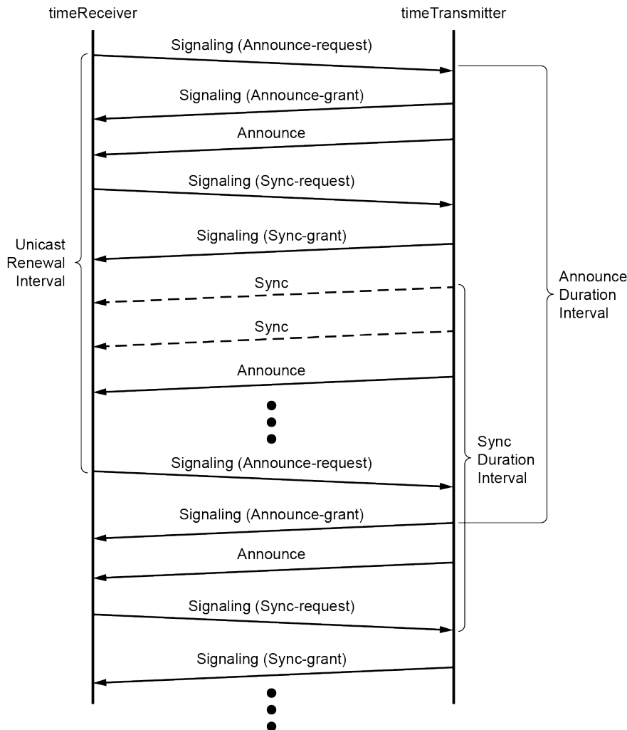
Figure 9: Message sequence between the PTP timeReceiver clock and PTP timeTransmitter clock
