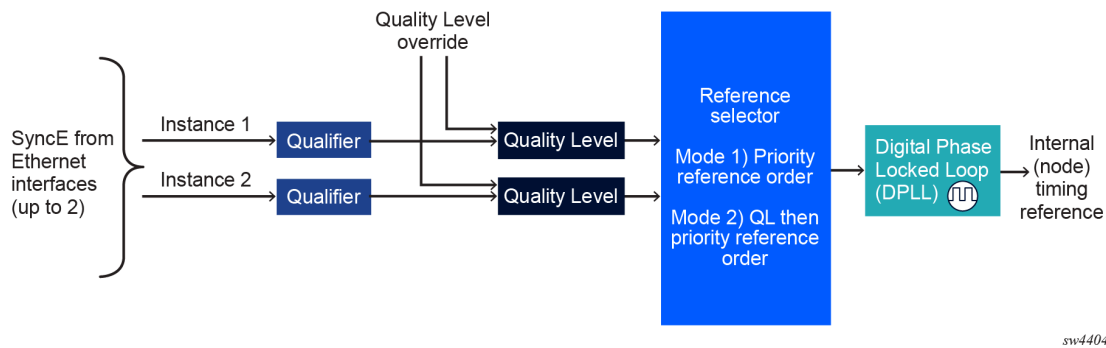
Figure 2: Logical model of the synchronization reference selection (7250 IXR-X1b/X3b)
