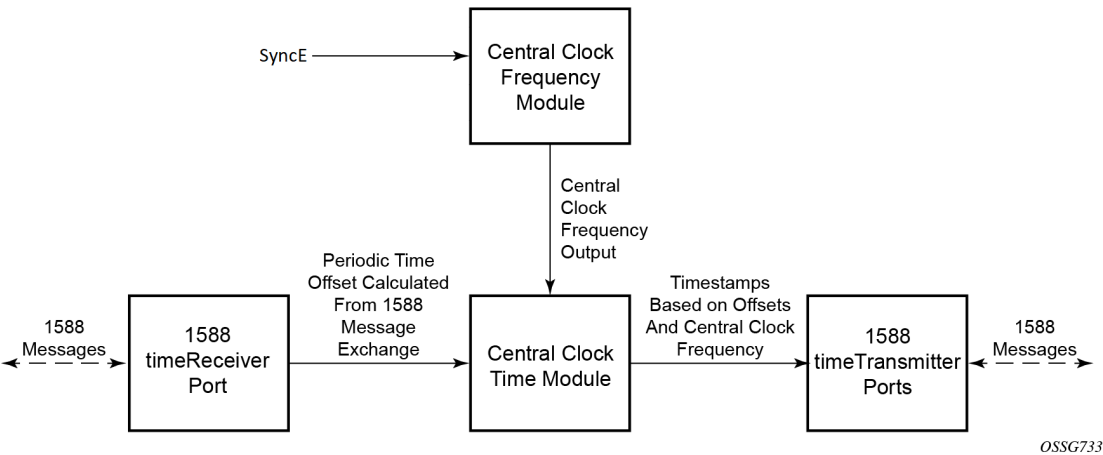
Figure 11: Logical model for using PTP/1588 for network synchronization
