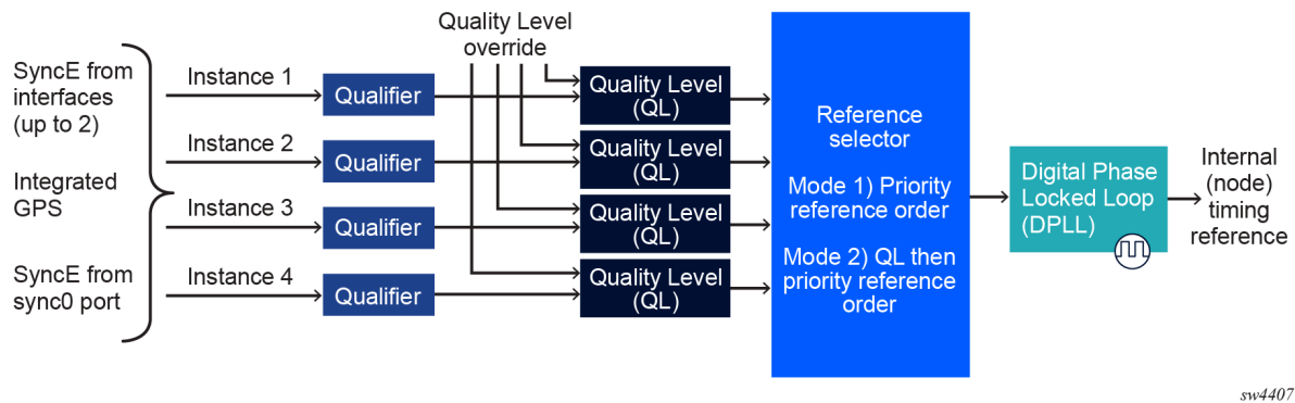
Figure 4: Logical mode of the synchronization reference selection (7730 SXR-1d-32D)
