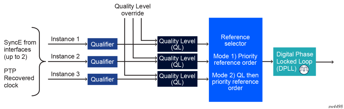
Figure 3: Logical model of the synchronization reference selection (7220 IXR-D5)
