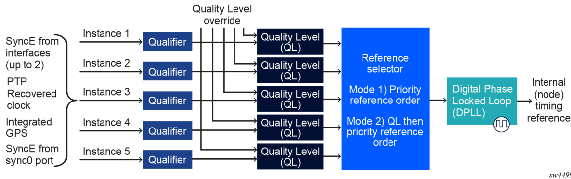
Figure 5: Logical mode of the synchronization reference selection (7730 SXR-1x-44s)
