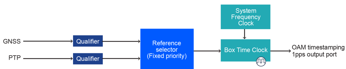
Figure 6: Default time reference selection
