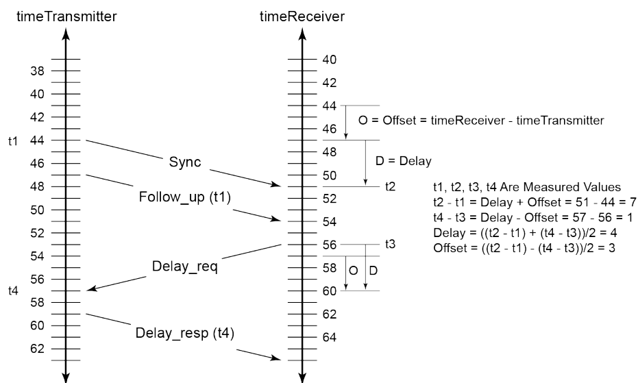
Figure 10: PTP timeReceiver clock and timeTransmitter clock synchronization timing computation
