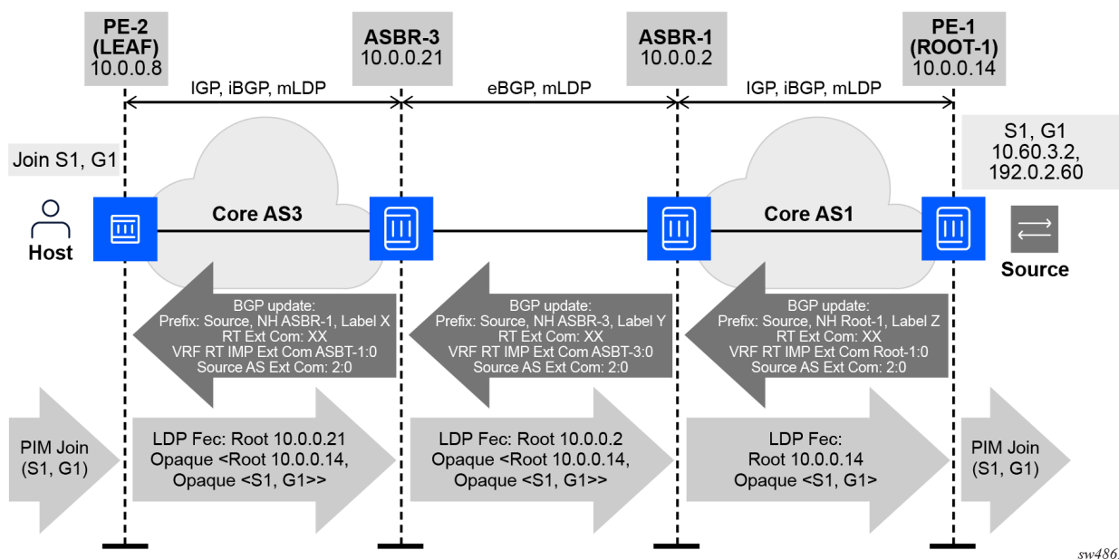
Figure 7: Non-Segmented Inter-AS mLDP setup
