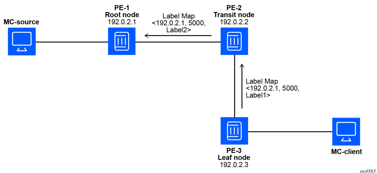
Figure 6: Setup of mLDP P2MP LSP
