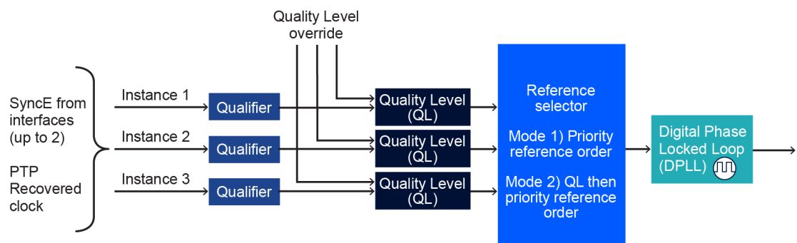
Figure 2: Logical model of the synchronization reference selection (7220 IXR-D5, 7250 IXR 6e/10e, and 7250 IXR-X1b/X3b/X4)
