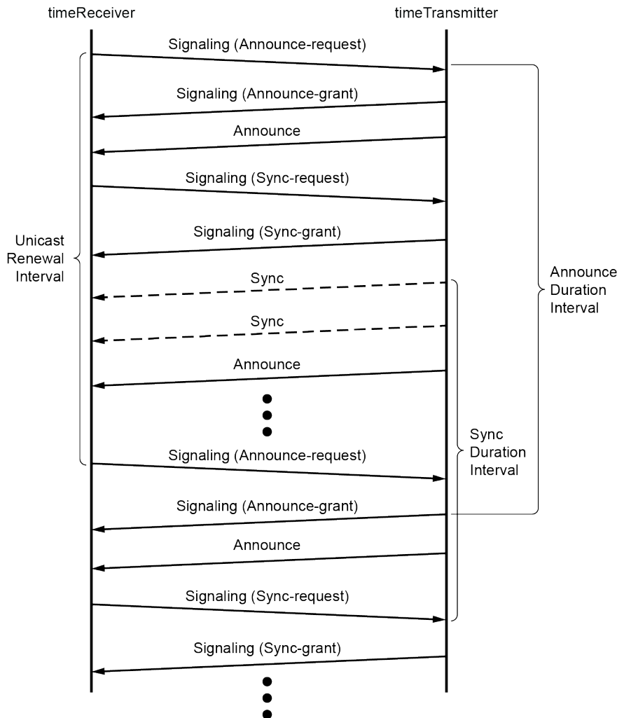
Figure 8: Message sequence between the PTP timeReceiver clock and PTP timeTransmitter clock
