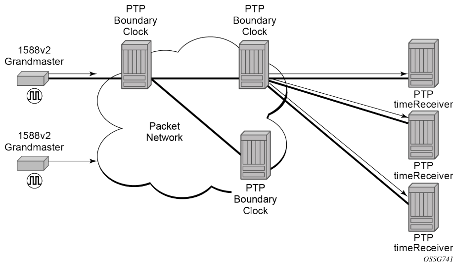
Figure 11: PTP boundary clock
