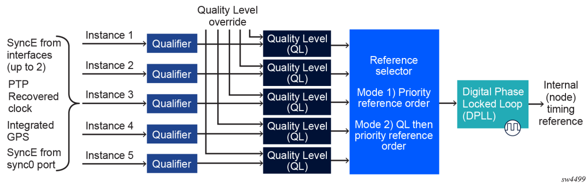
Figure 4: Logical mode of the synchronization reference selection (7730 SXR-1x-44s)
