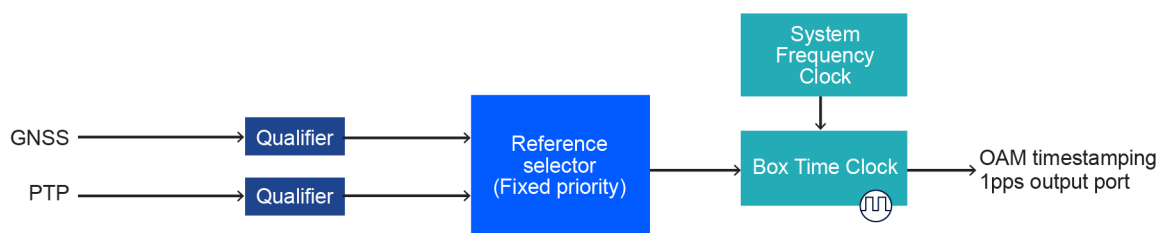
Figure 5: Default time reference selection
