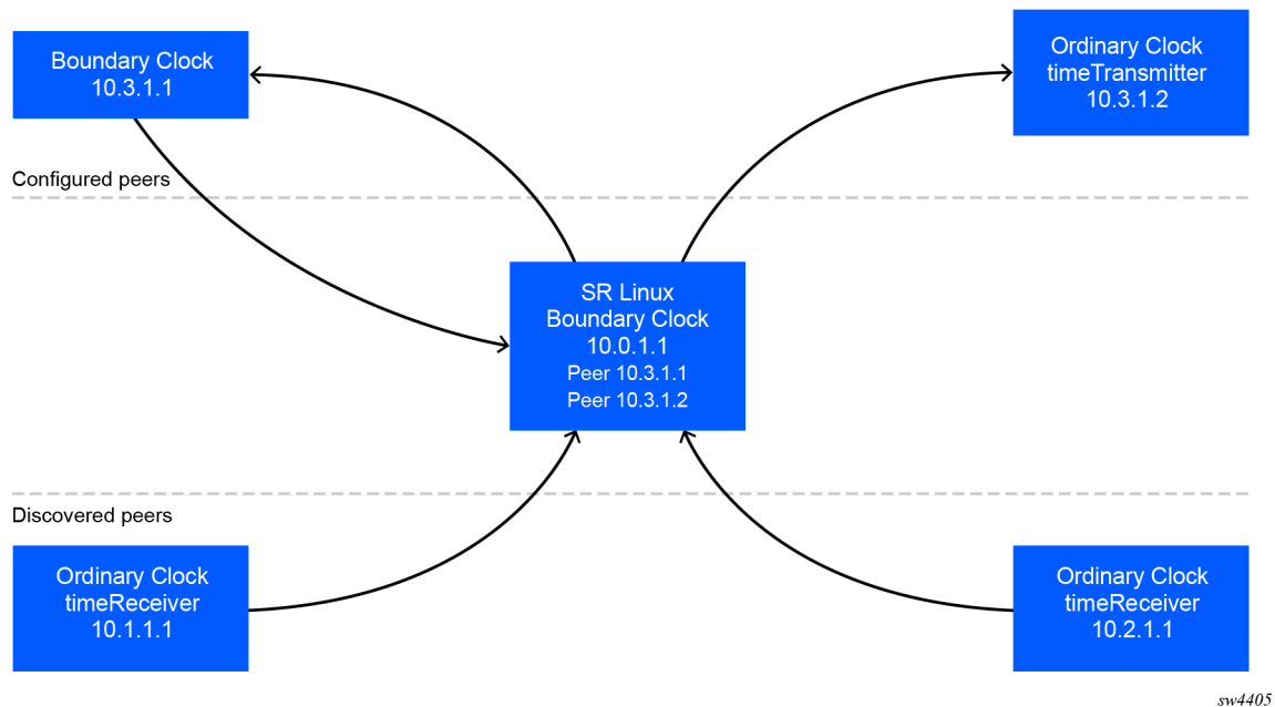
Figure 6: Peer clocks
