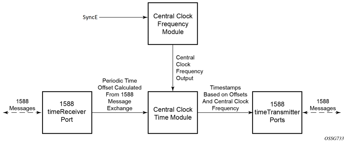
Figure 10: Logical model for using PTP/1588 for network synchronization
