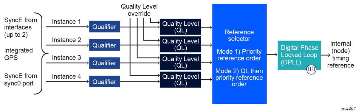
Figure 3: Logical mode of the synchronization reference selection (7730 SXR-1d-32D and 7730 SXR-1-32D)
