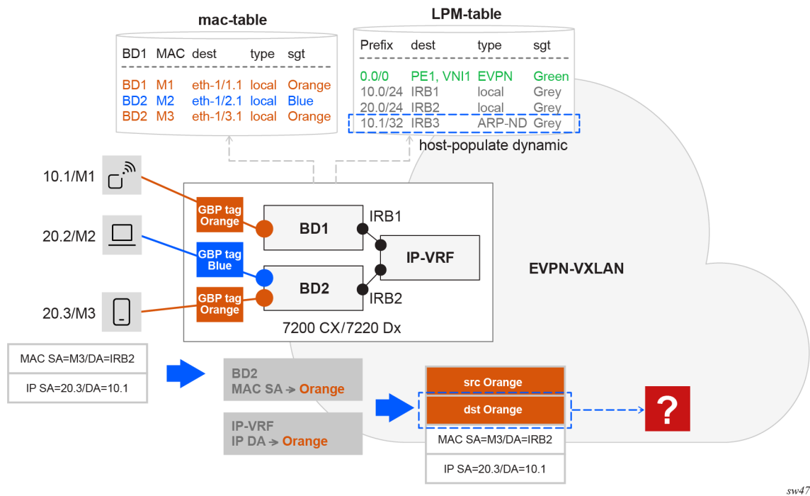
Figure 55: Assignment of GBP tag to ARP/ND host routes
