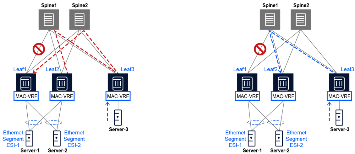
Figure 39: Underlay failure: default aliasing versus Anycast aliasing
