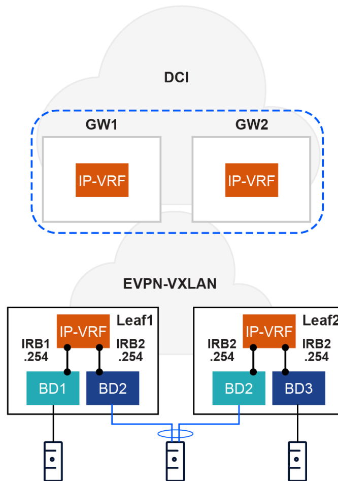
Figure 45: Multi-instance EVPN-IFL (MPLS-VXLAN) structure
