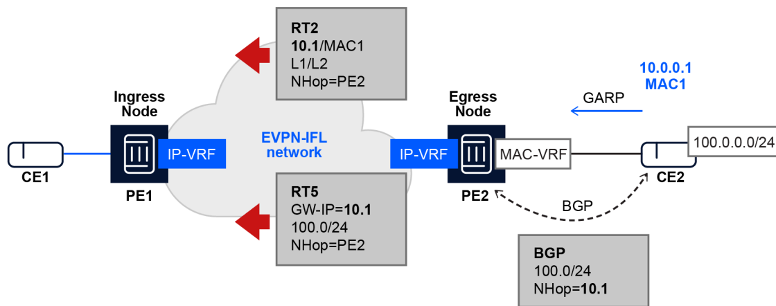
Figure 29: Recursive resolution of non-zero GW-IP prefix routes
