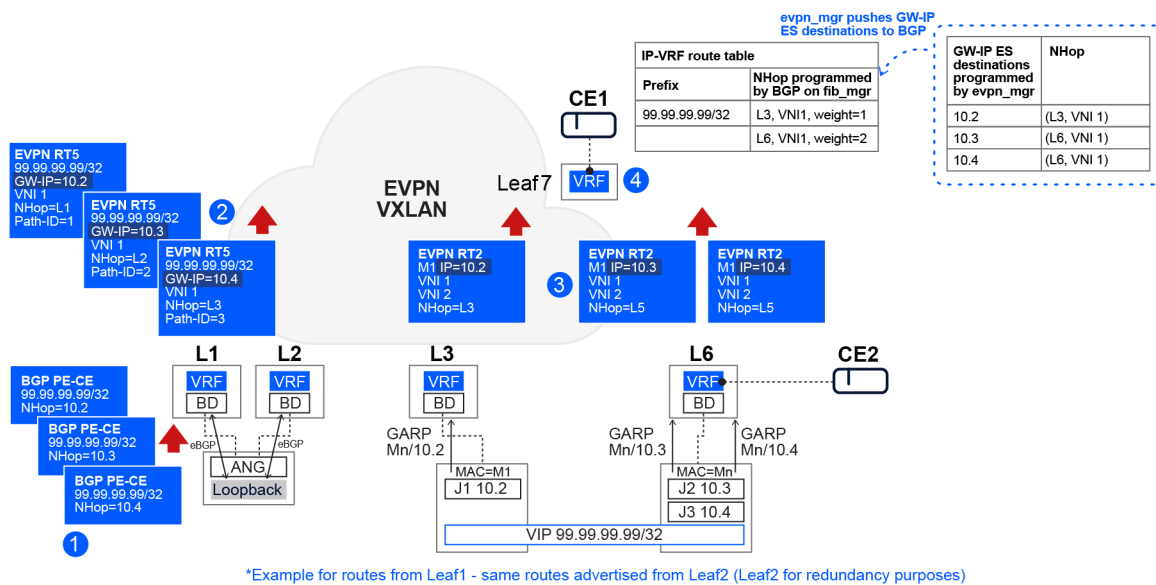
Figure 30: Gateway IP-based load balancing
