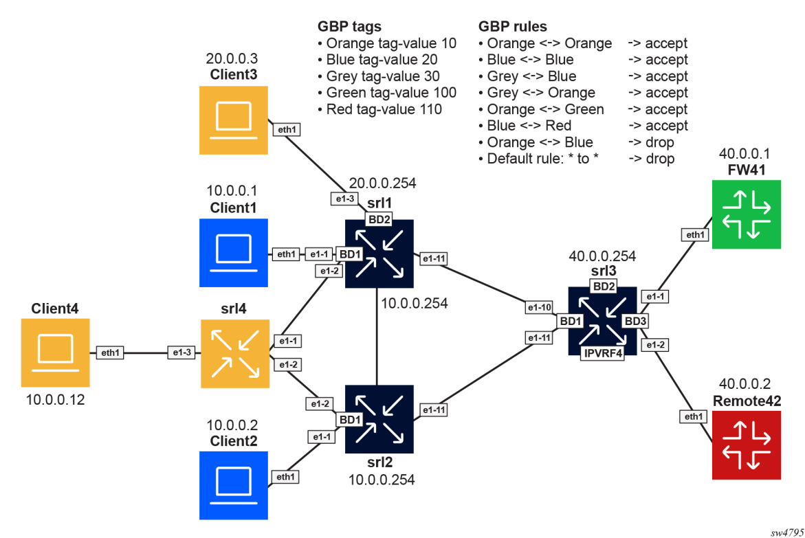
Figure 59: Centralized IRB EVPN VXLAN topology
