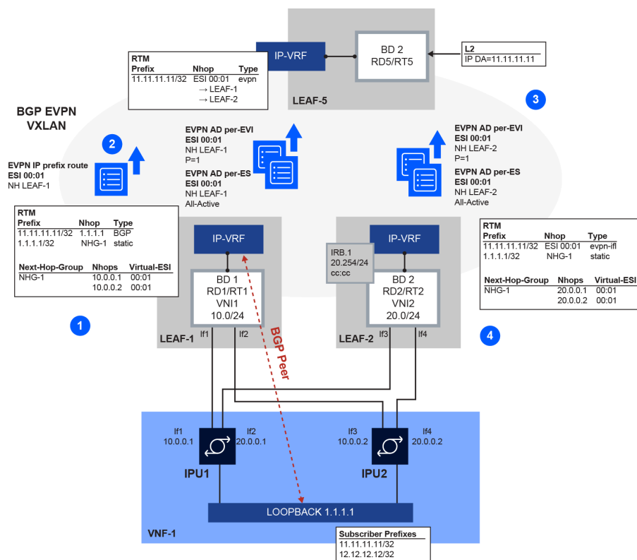
Figure 25: EVPN IP aliasing on SR Linux
