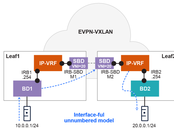
Figure 34: EVPN OISM example
