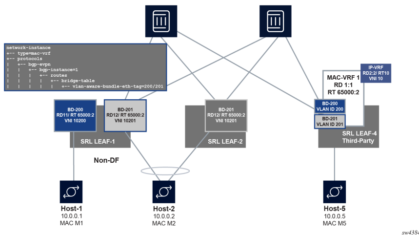
Figure 9: EVPN interoperability with VLAN-aware bundle services
