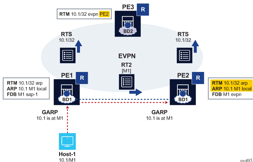
Figure 21: EVPN host route mobility
