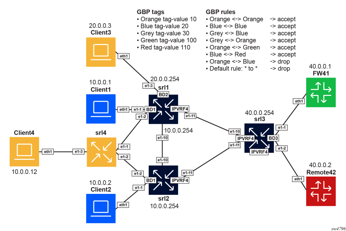
Figure 60: Distributed IRB EVPN VXLAN topology
