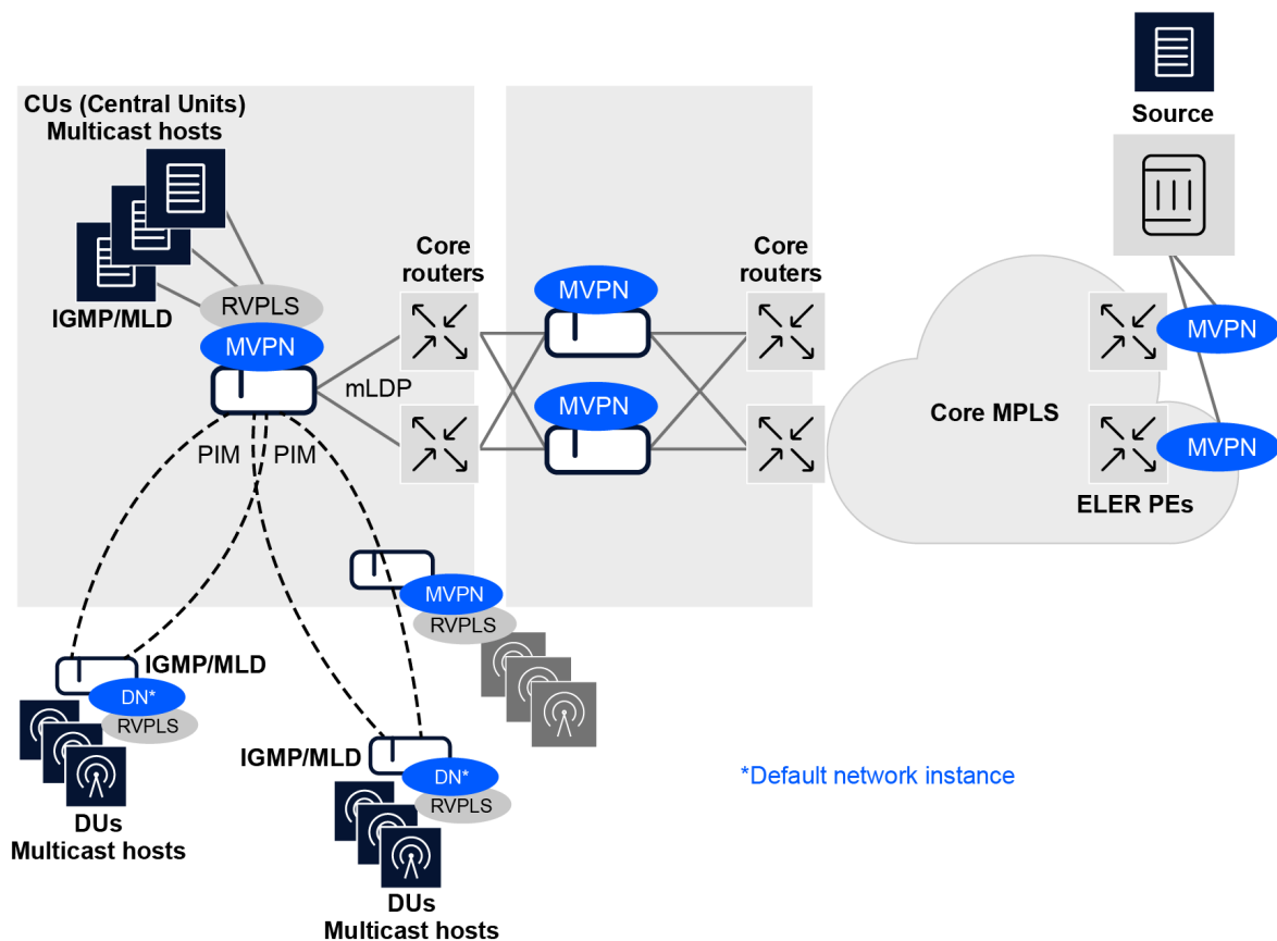
Figure 43: NG-MVPN control plane and protocol overview
