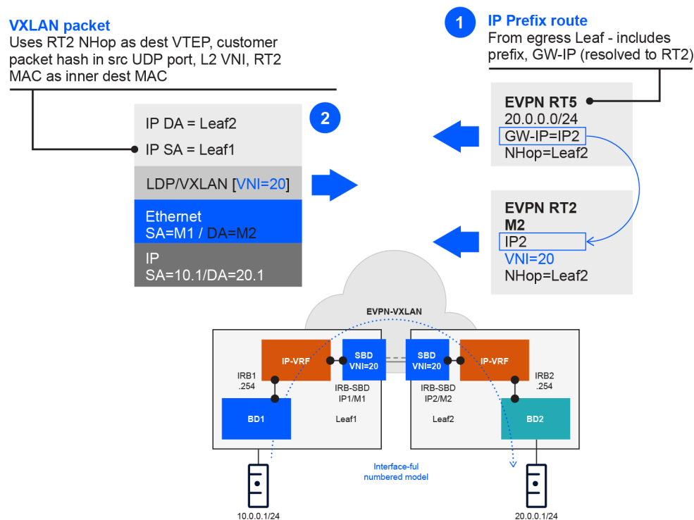
Figure 16: EVPN IFF numbered model
