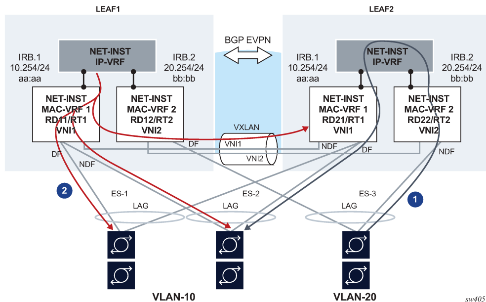
Figure 20: EVPN-VXLAN Layer 3 model – multihoming and anycast gateway
