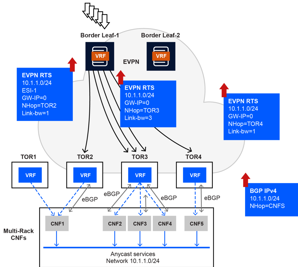
Figure 28: EVPN using weighted ECMP
