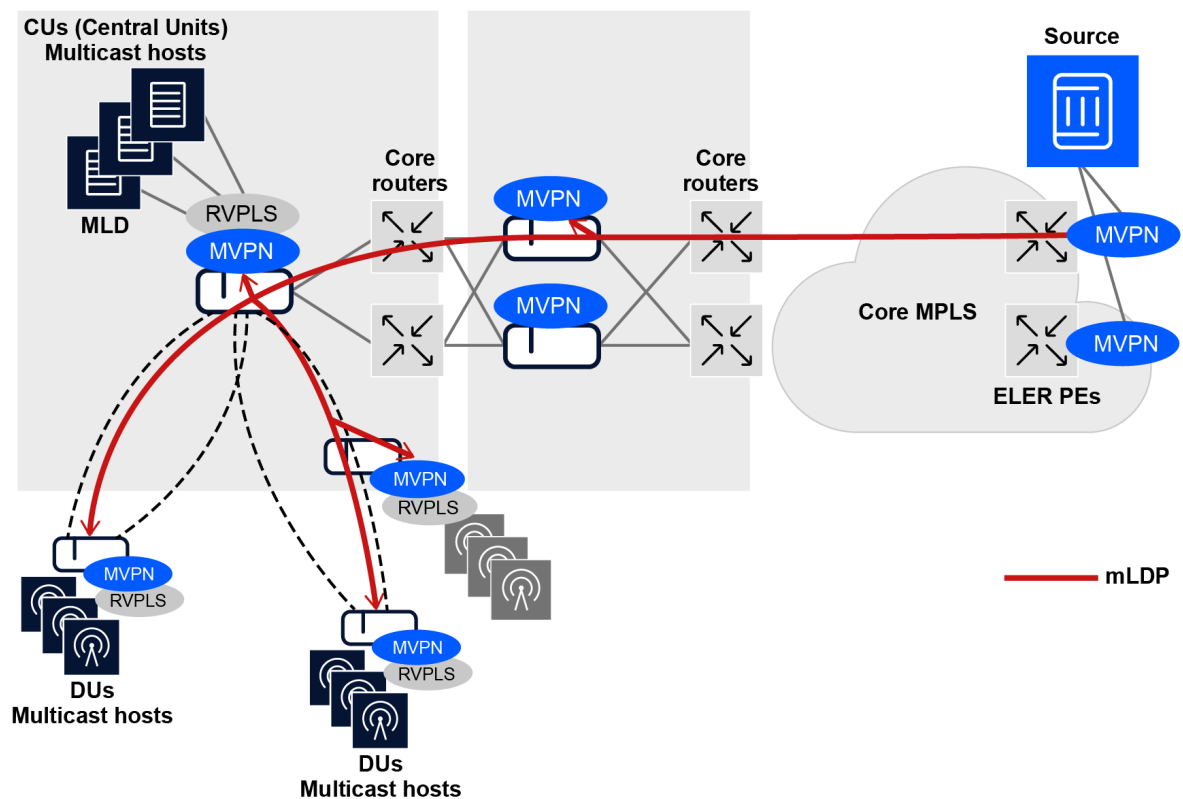
Figure 42: NG-MVPN with PIM, IGMP/MLD and mLDP signaling
