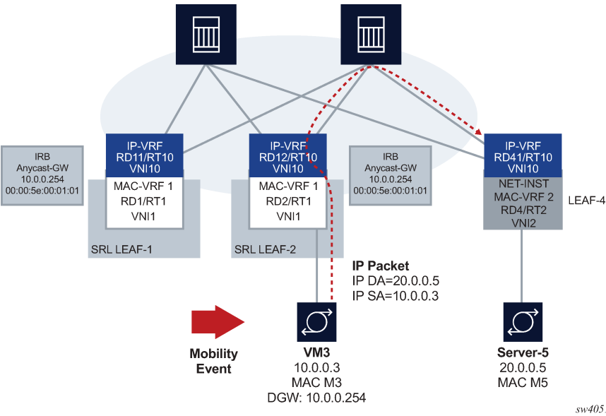
Figure 19: Anycast-GW IRB configuration
