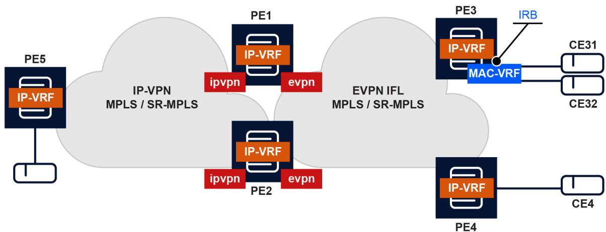
Figure 44: Multi-instance IP-VRF structure
