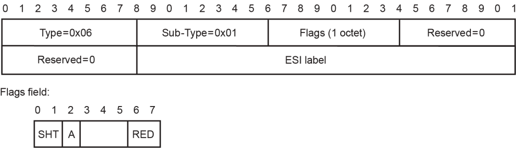
Figure 37: ESI label extended community
