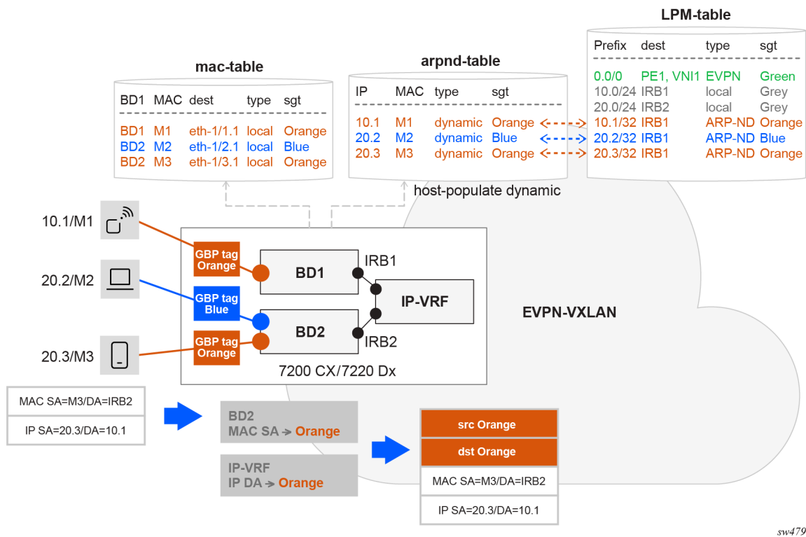
Figure 56: Propagation of tags to ARP/ND binds and host routes
