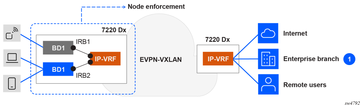
Figure 57: Enforcement in an EVPN distributed IRB model
