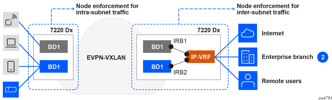
Figure 53: Centralized IRB model
