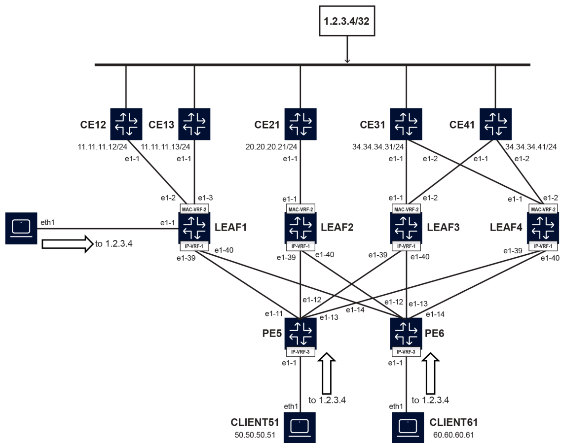
Figure 50: Combined ECMP
