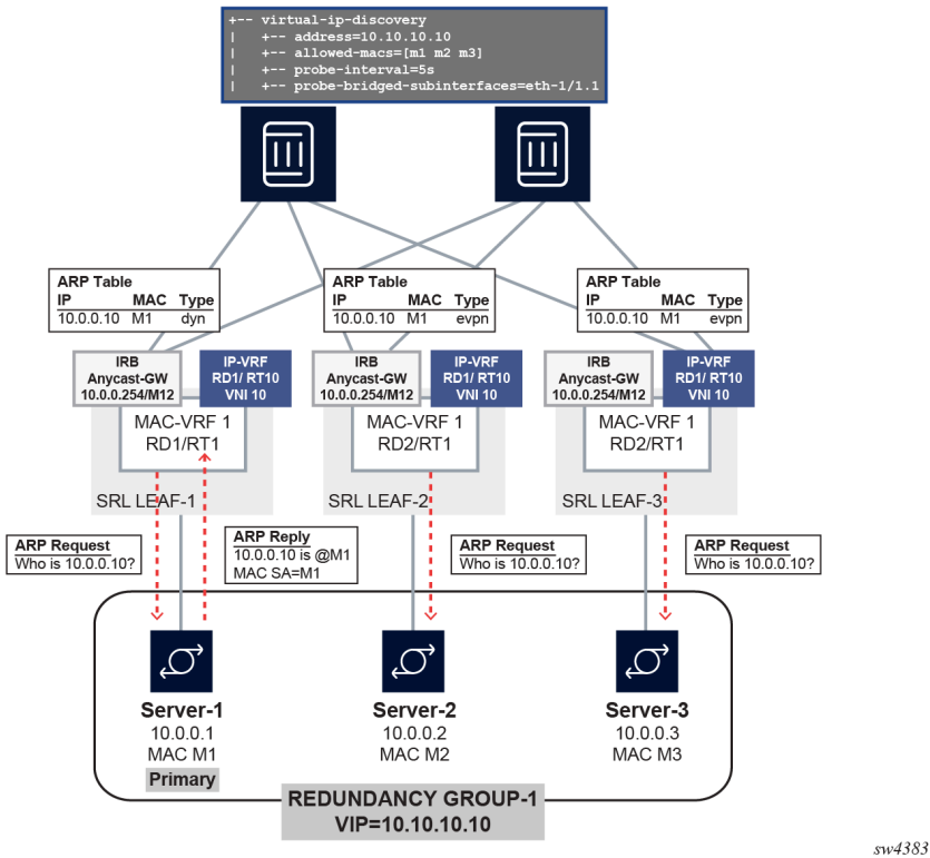
Figure 22: VIP discovery for the active server in a server group
