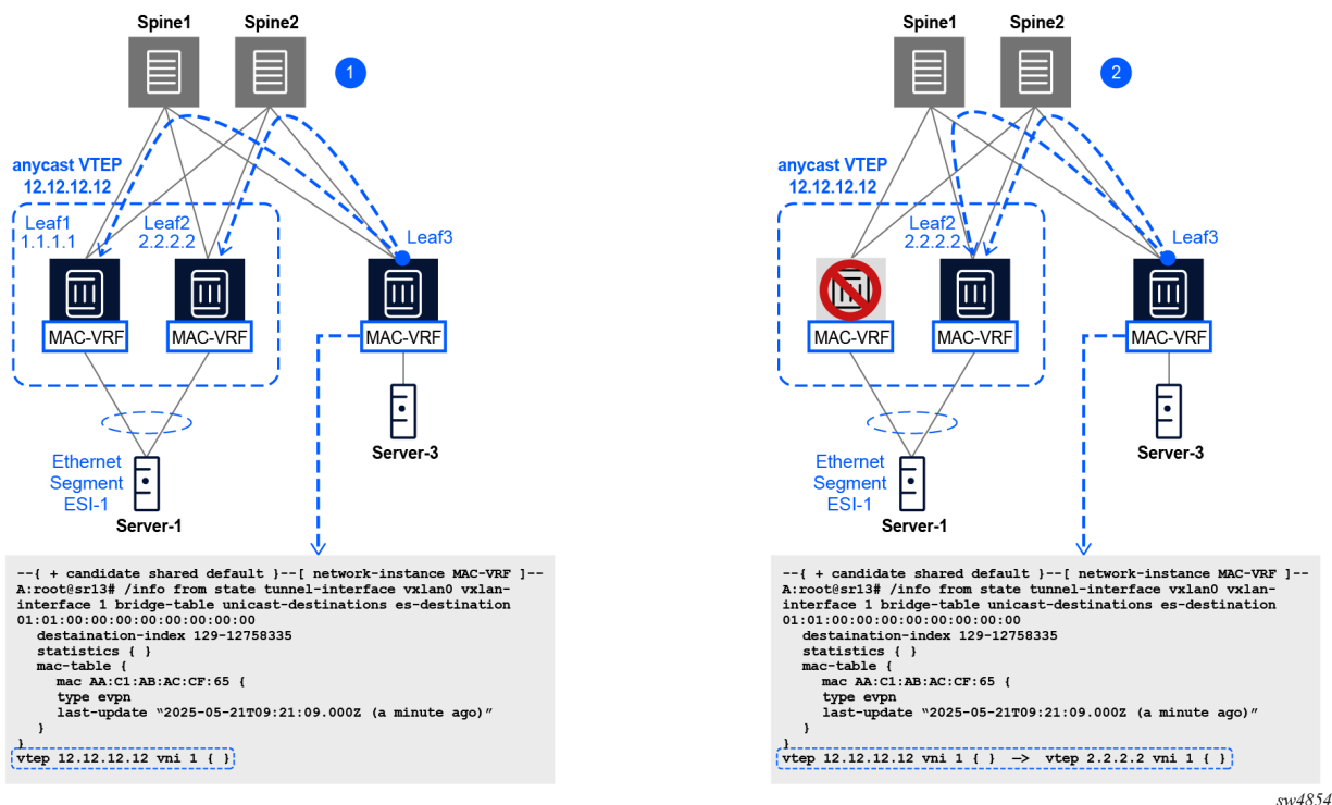
Figure 40: Egress leaf node failure behavior in Anycast ESes
