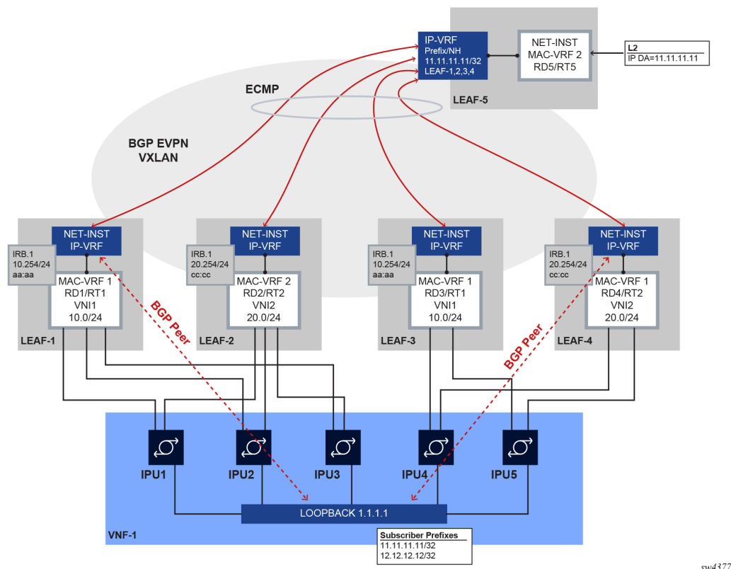
Figure 24: BGP peering to VNF loopback
