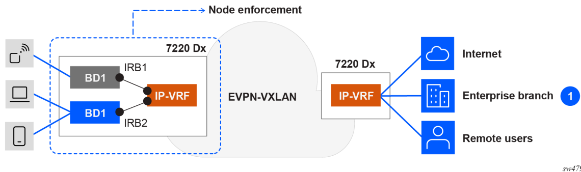
Figure 52: Distributed IRB model for micro-segmentation
