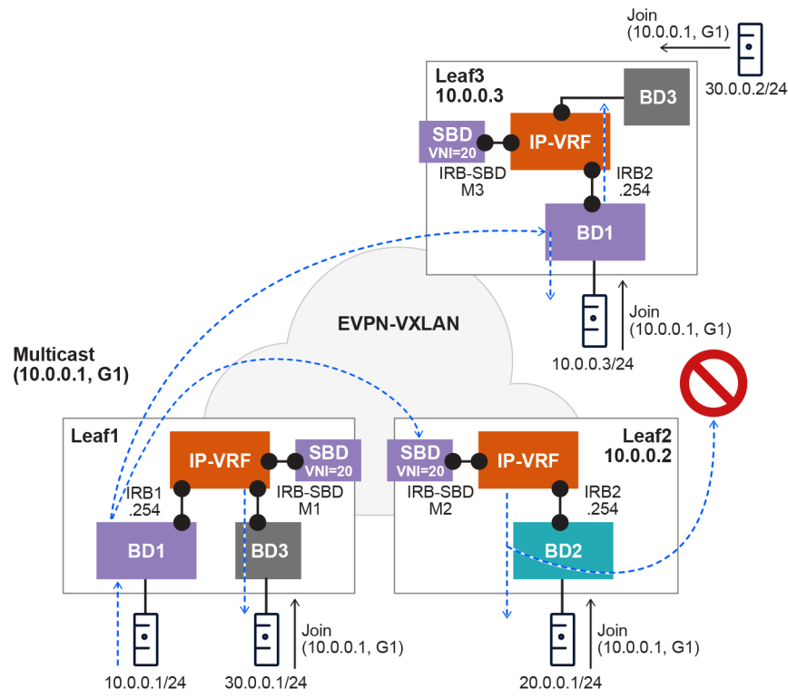
Figure 33: OISM data path perspective
