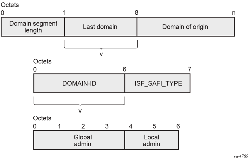
Figure 48: D-PATH attribute
