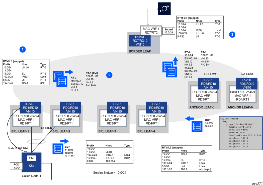
Figure 27: Centralized routing model
