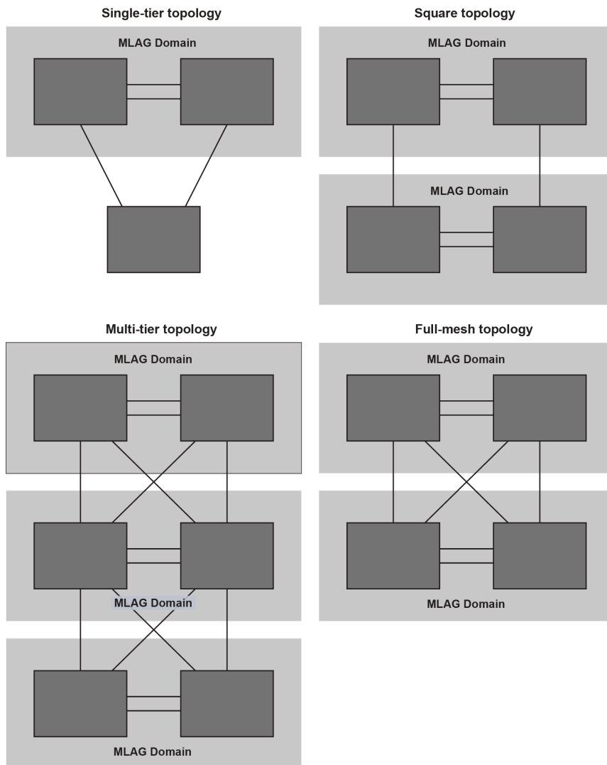
Figure 65: MLAG topologies
