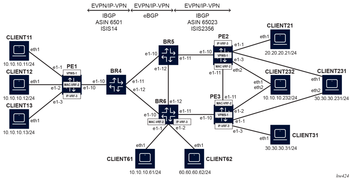
Figure 49: EVPN and IP-VPN services on inter-AS option B
