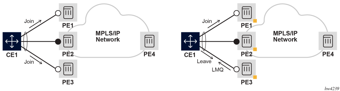
Figure 31: Multicast state synchronization for EVPN MH
