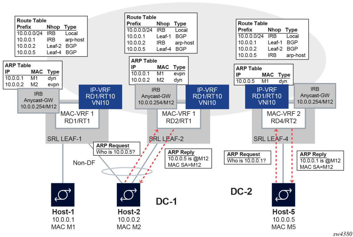
Figure 23: Layer 3 Proxy ARP/ND
