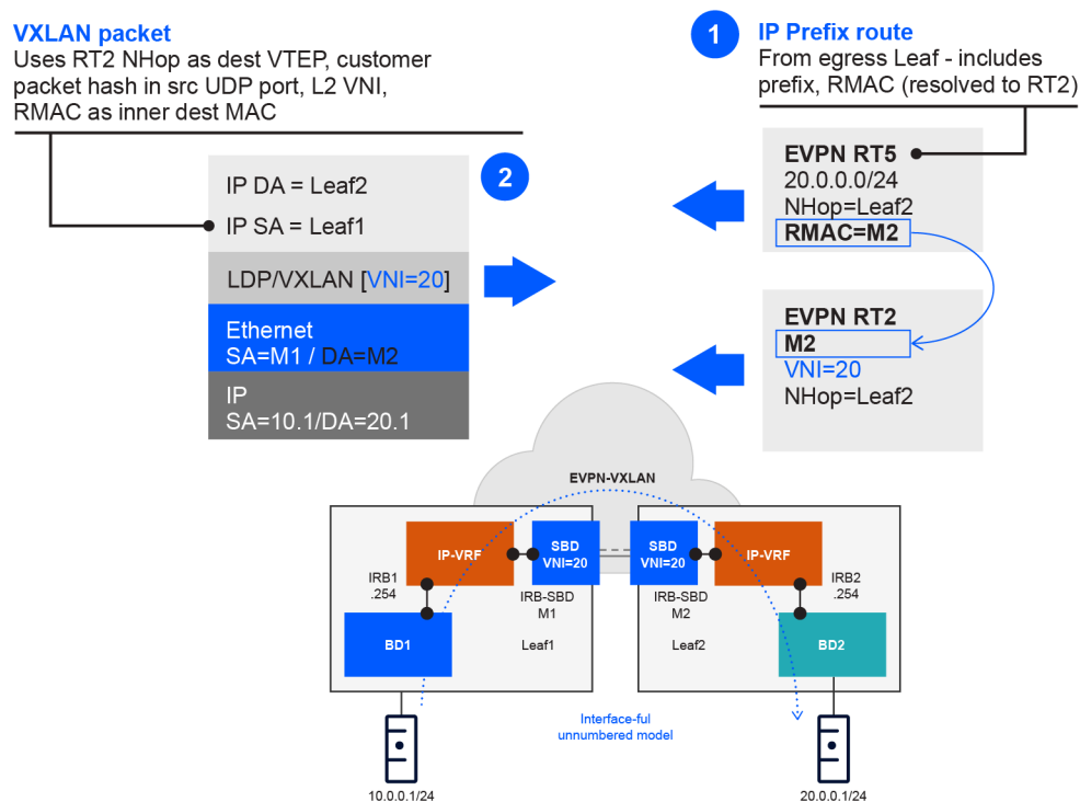
Figure 17: EVPN IFF unnumbered model
