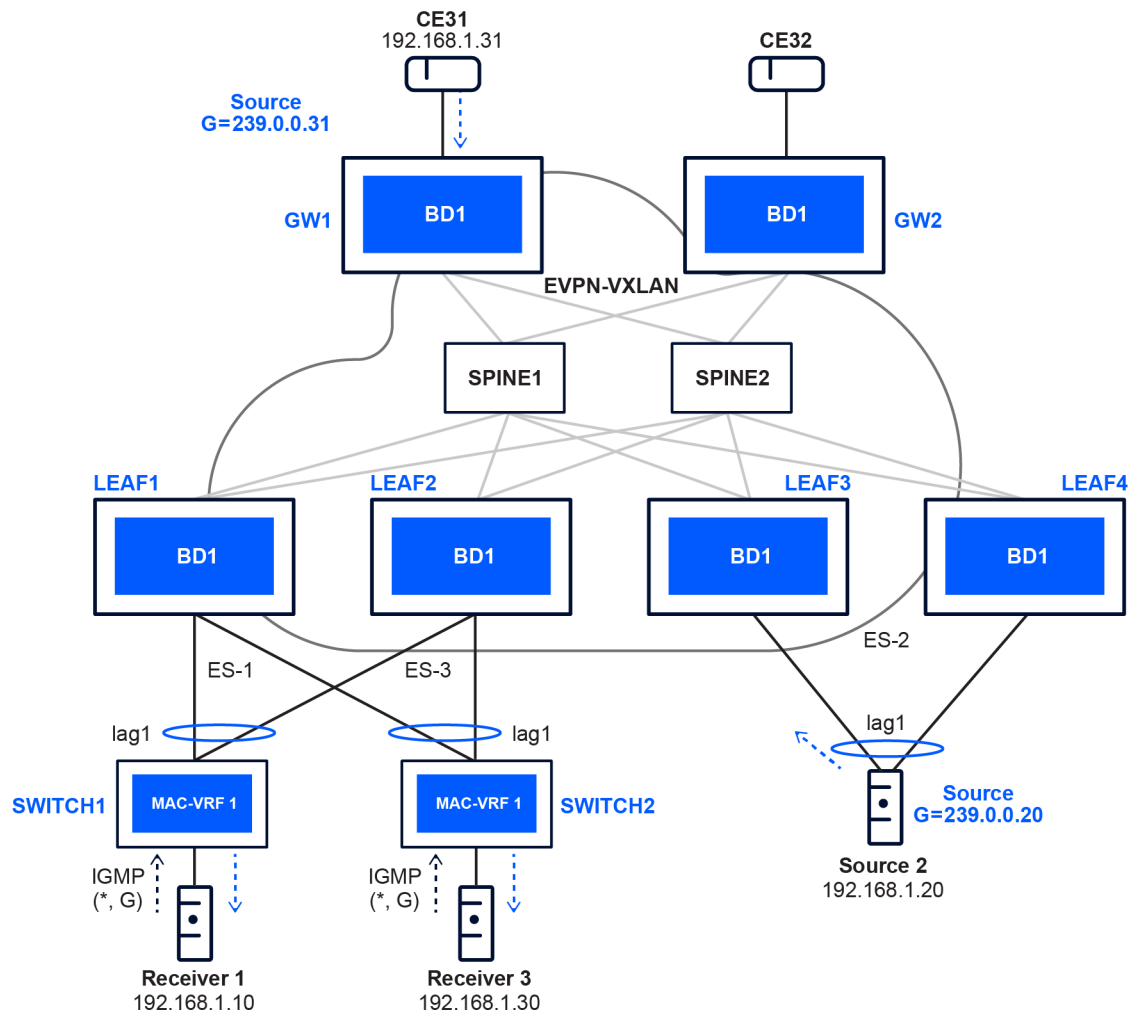
Figure 32: EVPN multicast for Layer 2
