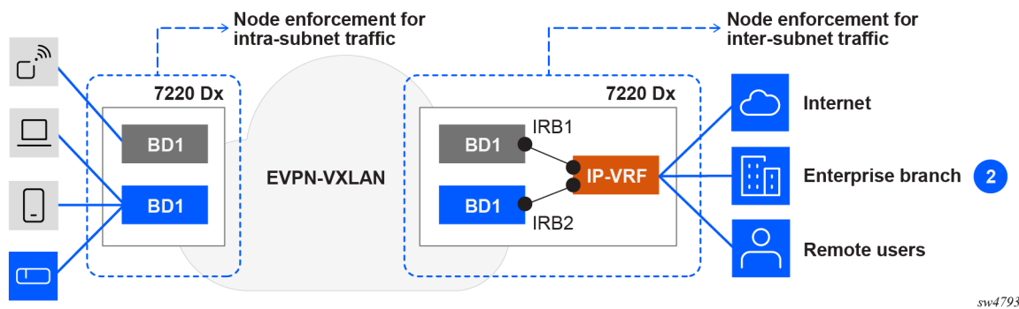
Figure 58: Enforcement in an EVPN centralized IRB model
