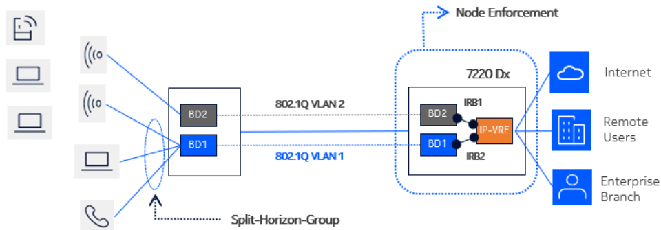
Figure 54: Centralized IRB model for Layer 2 aggregation
