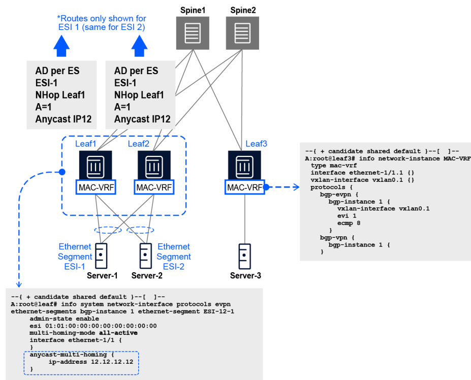
Figure 36: EVPN Anycast MH
