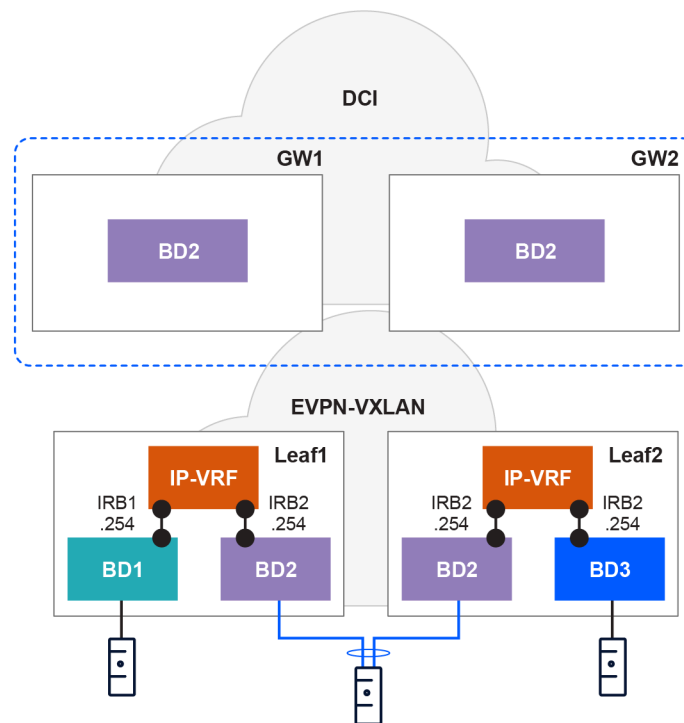
Figure 46: Multi-instance MAC-VRF structure
