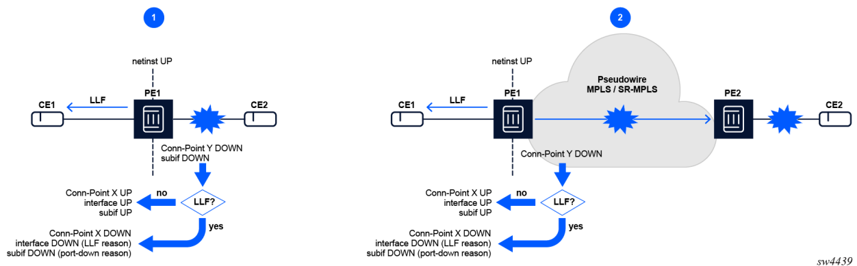
Figure 11: LLF in VPWS network instances
