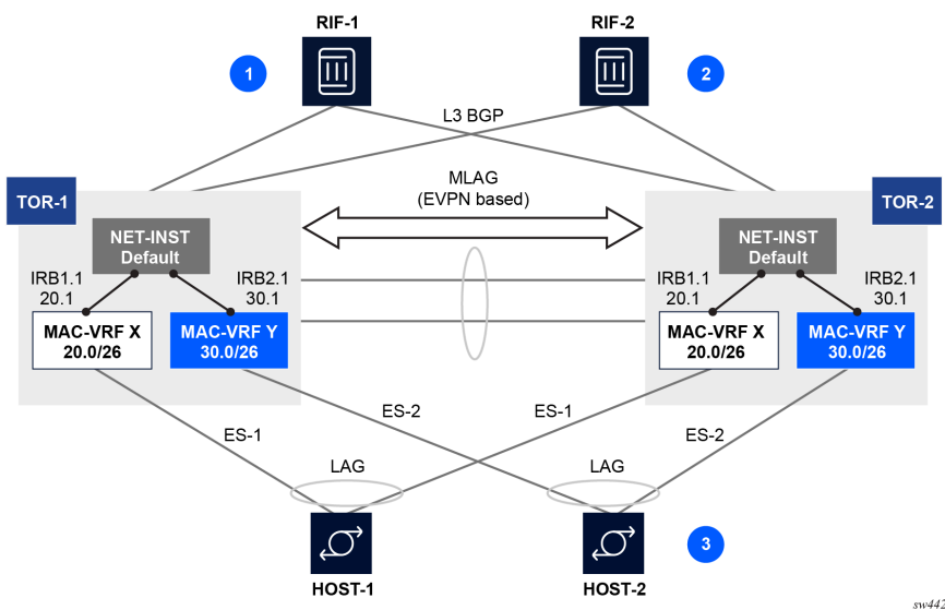
Figure 62: Active-active connectivity example
