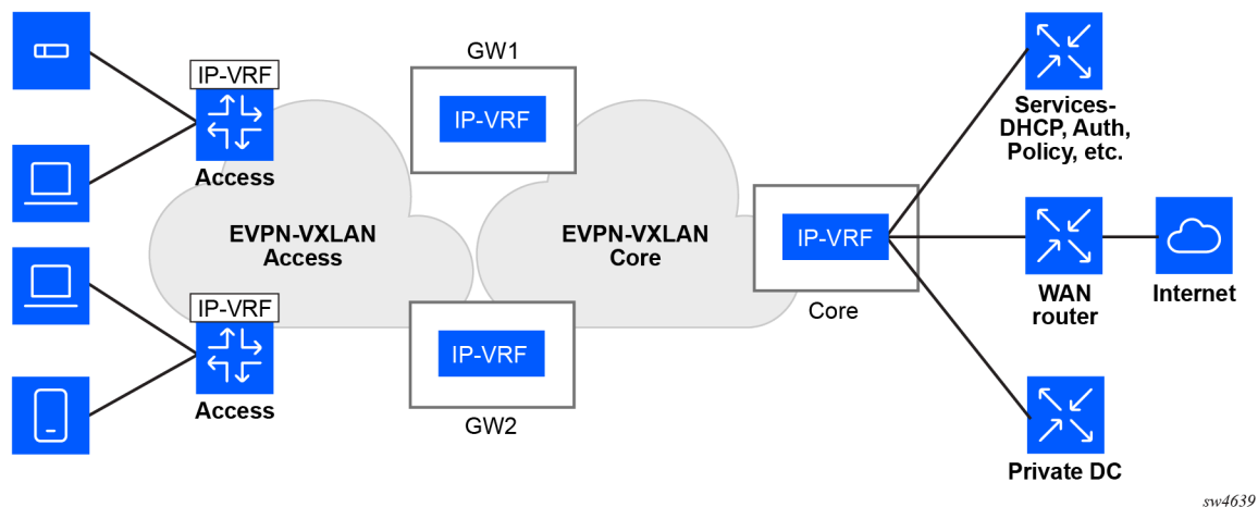
Figure 47: Inter-domain Layer 3 solution
