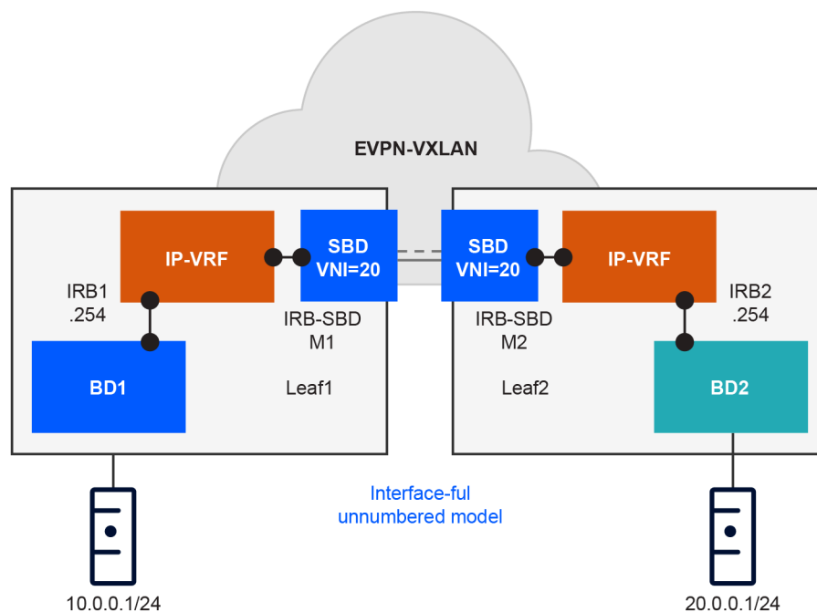
Figure 18: EVPN IFF implementation
