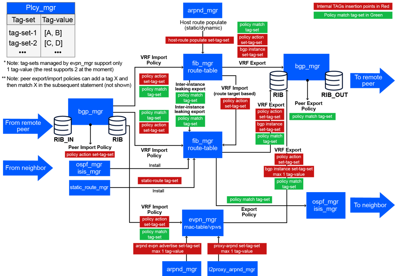
Figure 35: Applications for internal tags, insertion points, and policy points
