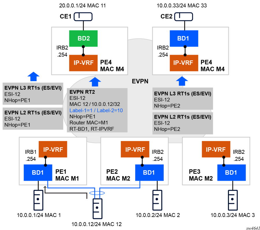
Figure 26: IP aliasing for BGP-EVPN-IFL host routes
